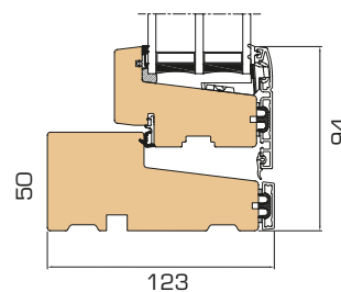
3 Vertical section sill
